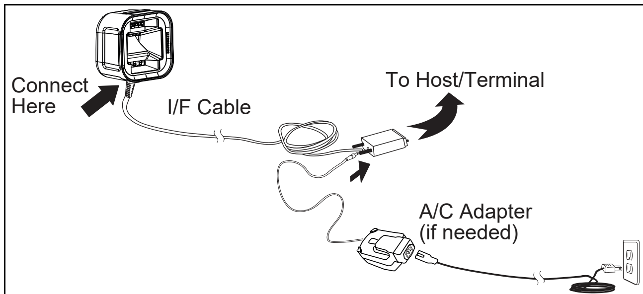
Figure 1. Connecting the Scanner
