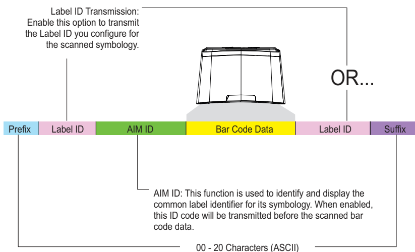
Figure 5. Breakdown of a Message String
