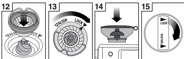
Push upper burr firmly into position
