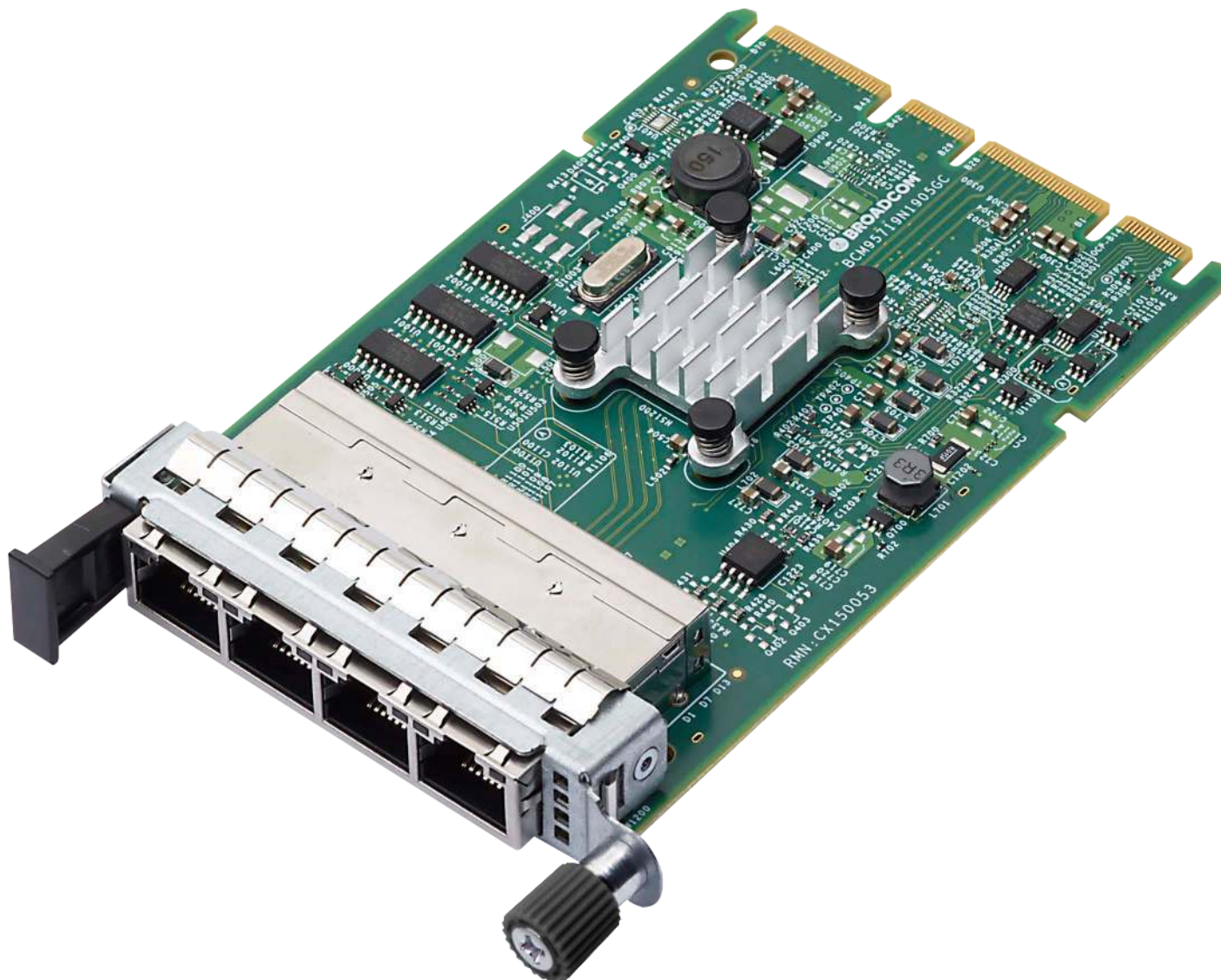
Figure 1: BCM95719N1905C OCP 3.0 SFF Card
