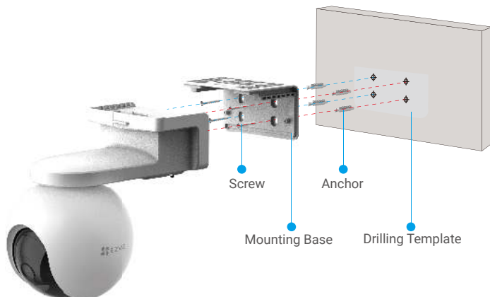
Fig. 2 Wall Mount
