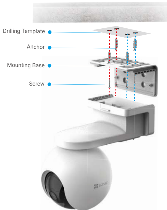
Fig. 1 Ceiling Mount
