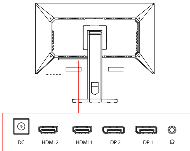
Figure 4-1 Input and output interface
