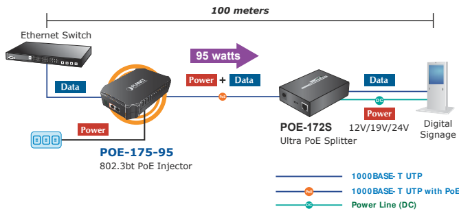
Figure 3: Architecture of connected POE-175-95 and POE-172S
