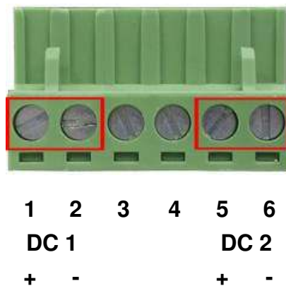
Figure 2-15 6-pin Terminal Block Power Wiring Input for IGS-5225-16T4S & IGS-5225-20T4C2X
