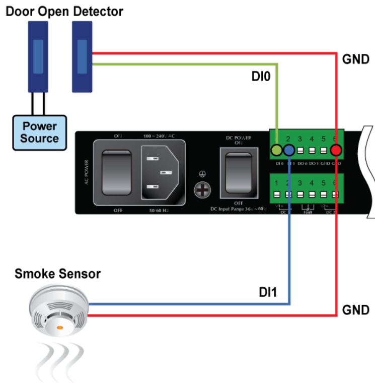
Figure 2-18 Wires DI0 and DI1 to Open Detector
