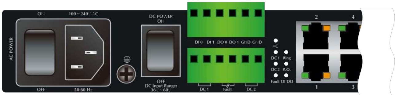
Figure 2-9: IGS-5225-16T4S LED on Front Panel
