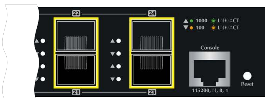
Figure 2-12: IGS-5225-24P4S LED on Front Panel
