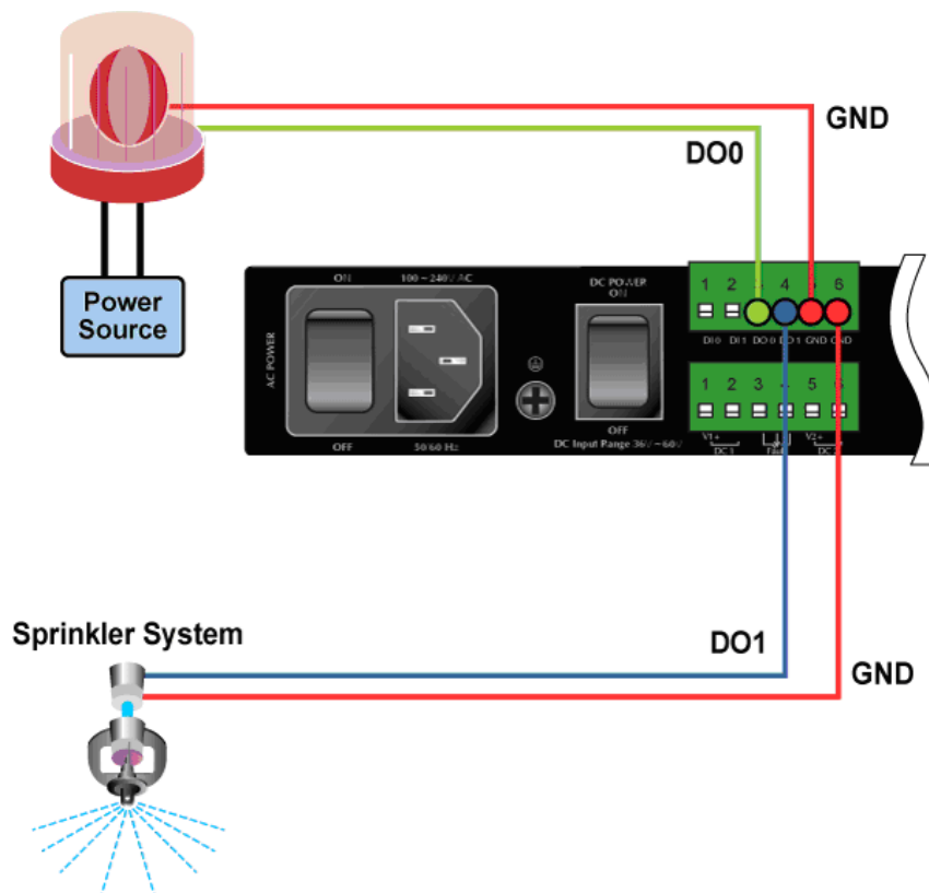
Figure 2-19 Wiring DO0 and DO1 to Open Detector
