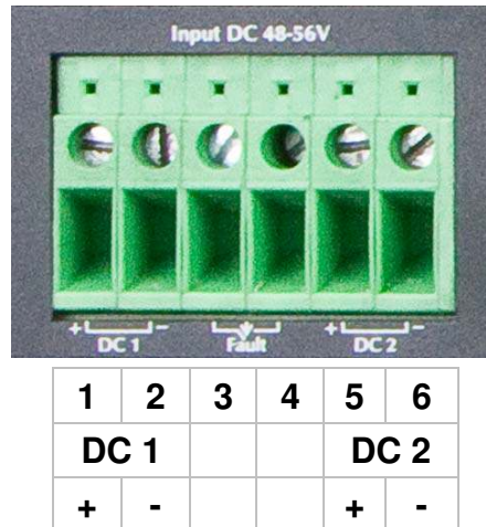
Figure 2-16 6-pin Terminal Block Power Wiring Input for IGS-5225-24P4S
