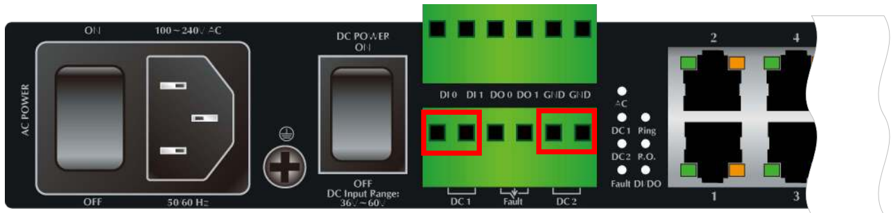
Figure 2-13: IGS-5225-16T4S & IGS-5225-20T4C2X Managed Switch Upper Panel
