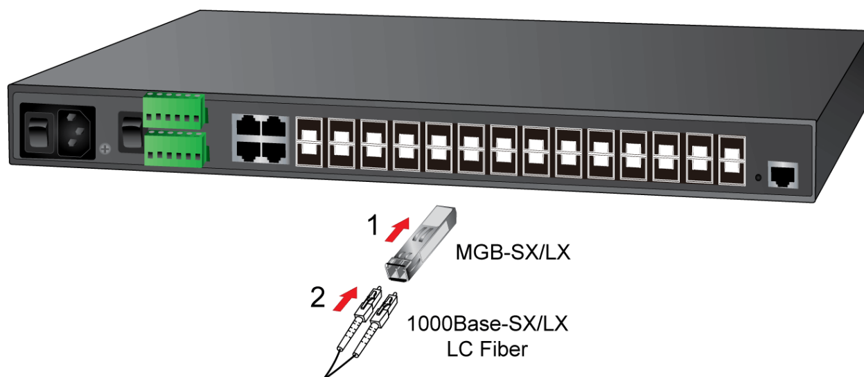
Figure 2-3-1: Plugging in the SFP Transceiver
