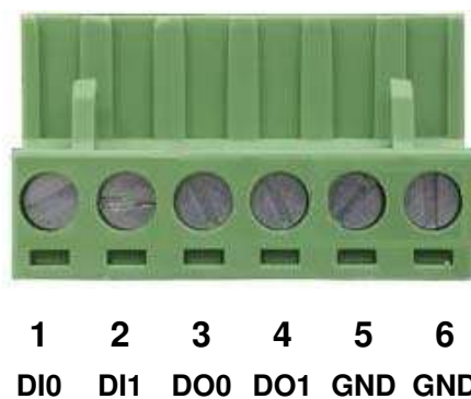
Figure 2-17 6-pin Terminal Block for DI and DO Wiring Input
