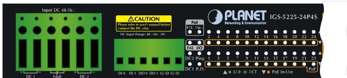
Figure 2-11: IGS-5225-24P4S LED on Front Panel
