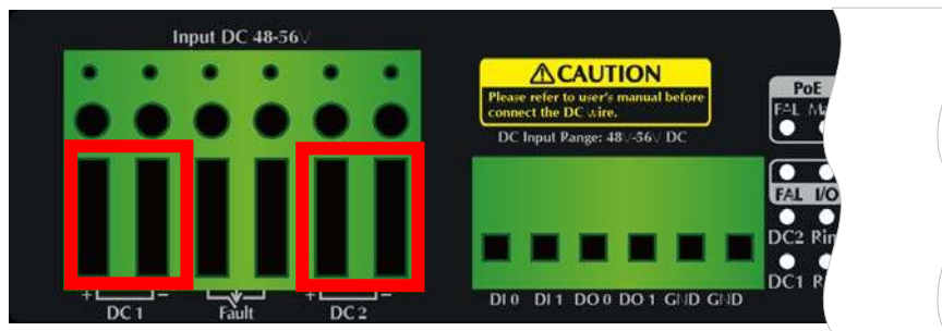
Figure 2-14: IGS-5225-24P4S Managed Switch Upper Panel
