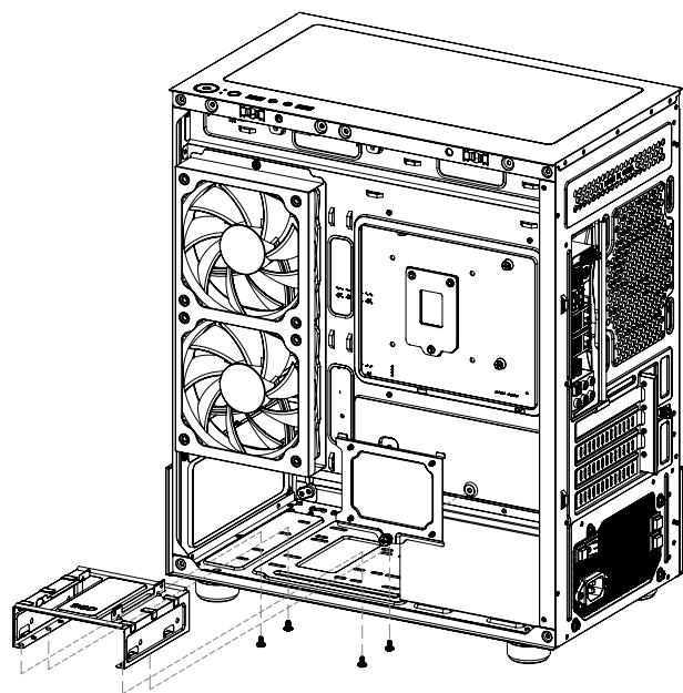
3.5" HDD
