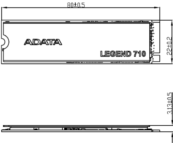
<With heatsink>
