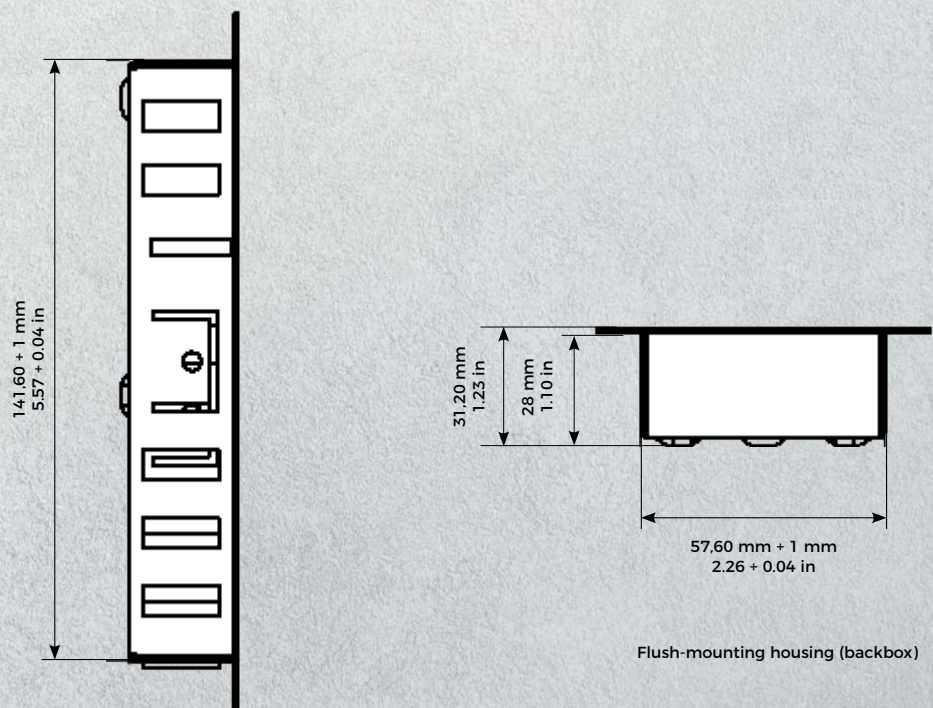
Flush-mounting housing (backbox)
