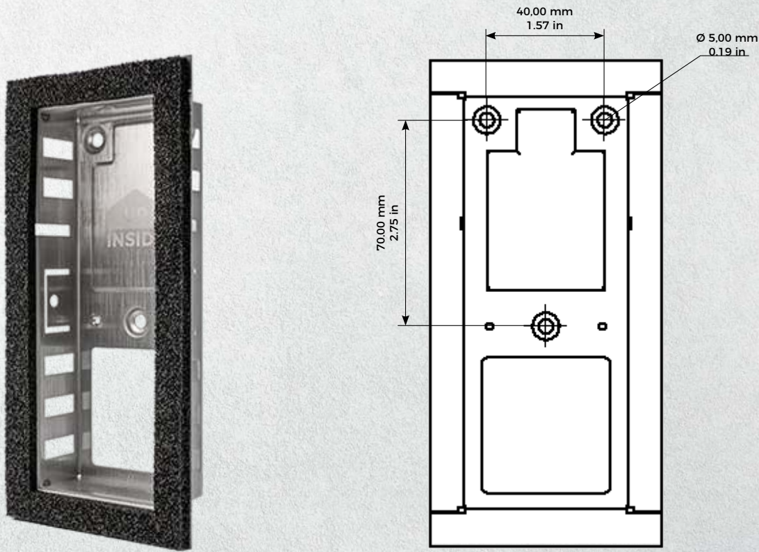
Flush-mounting housing (backbox)
