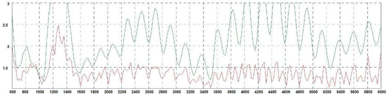
Typical VSWR*
