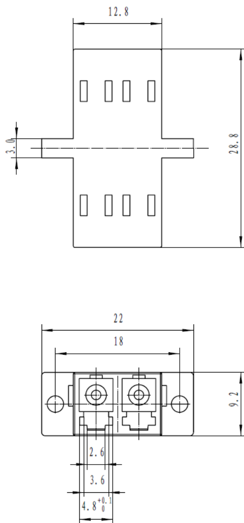
LC Duplex
