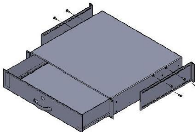
Explode View
