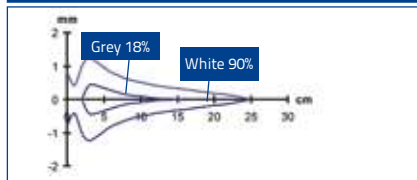
Detection area - radial
