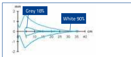
Detection area - axial
