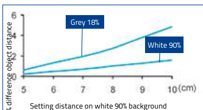
Detection difference with EASYtouch™ acquisition
