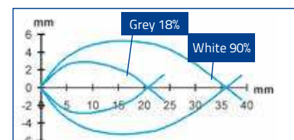
Detection area - proximity *
