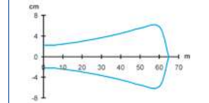
Detection area - axial
