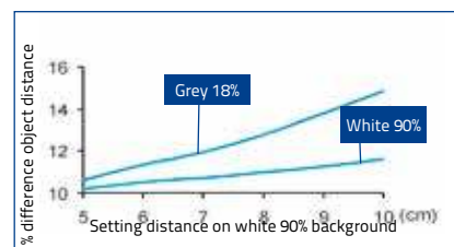
Detection difference with fine acquisition
