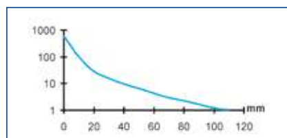
Excess gain - through beam *
