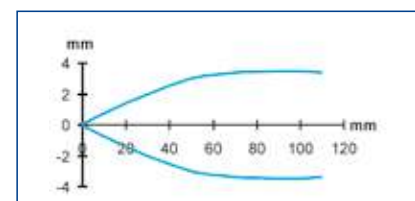
Detection area - through beam *
