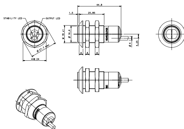
Cable version
