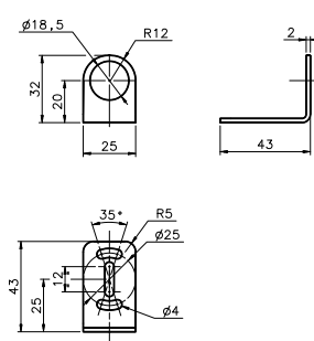
ST-5012
