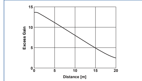
EXCESS GAIN
