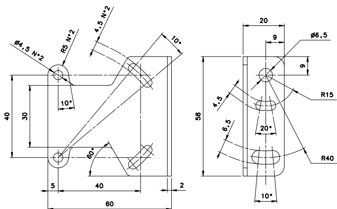
ST-504
