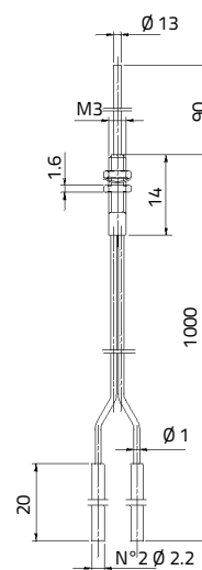
OF-44
