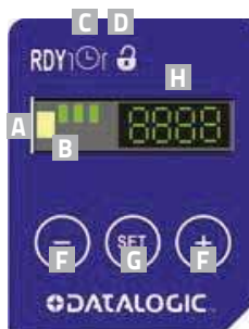
TL46-WLF ENHANCED
