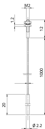
OF-42
