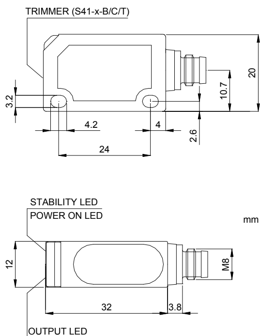
M8 CONNECTOR VERSION
