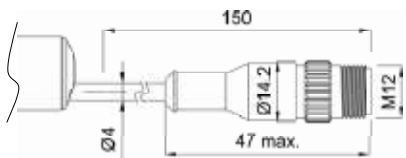
Pig-tail version
