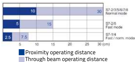
S7-2/5 proximity - Fast mode *
