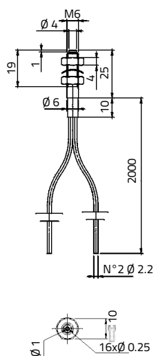
OF-36
