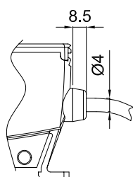
CABLE VERSION
