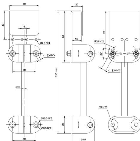
JOINT-60
