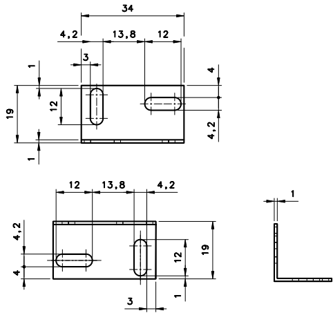
ST-505
