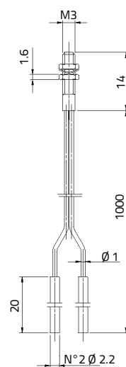
OF-43
