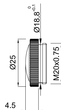
18 mm LENS
