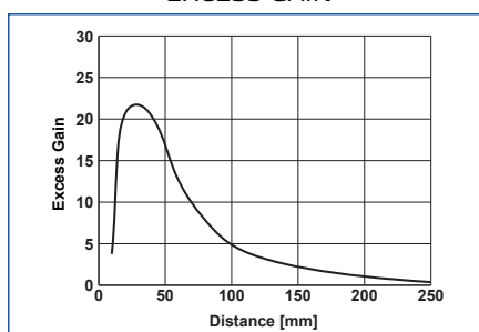
EXCESS GAIN
