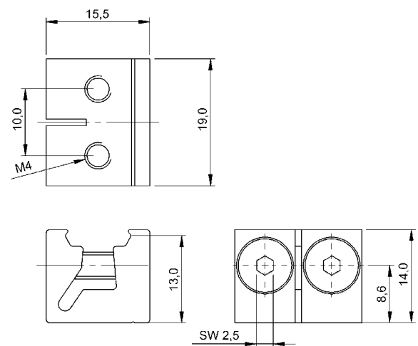
ST-5042
