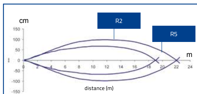
Polarized retroreflective on R2 reflector
