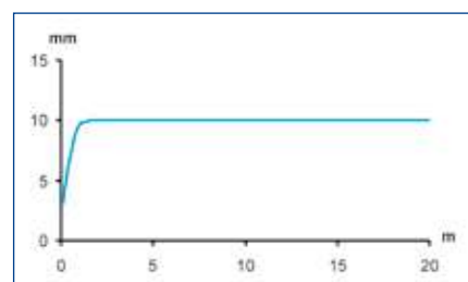
Resolution on R7 reflector
