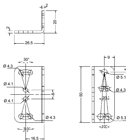
ST-5020
