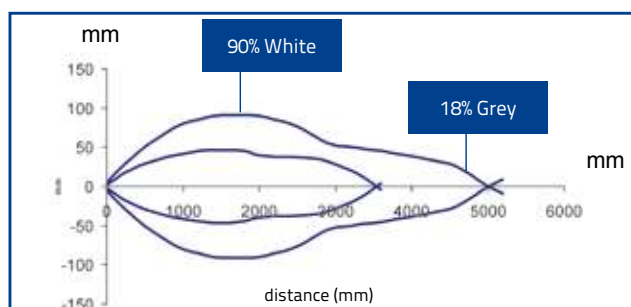
Diffuse proximity
