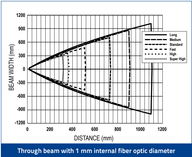
Detection area
