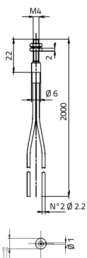
OF-38
