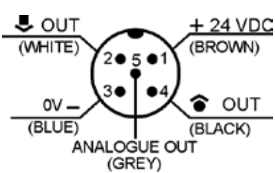
Distance S81-Y
