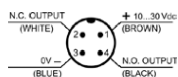
M12 CONNECTOR
