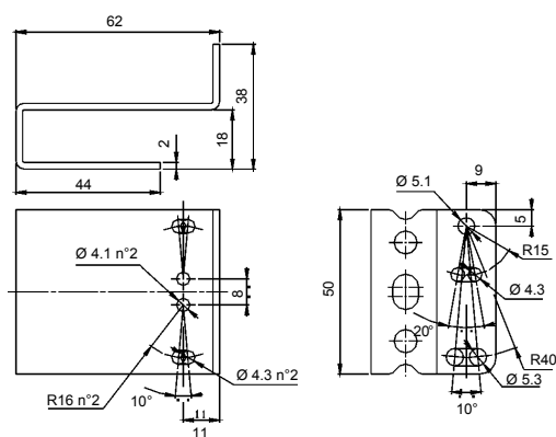
JOINT-60
