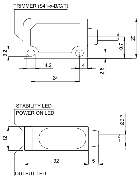
CABLE VERSION
