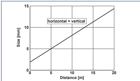
DETECTION SPOT SIZE
