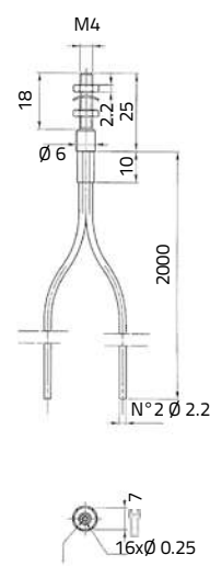
OF-44
