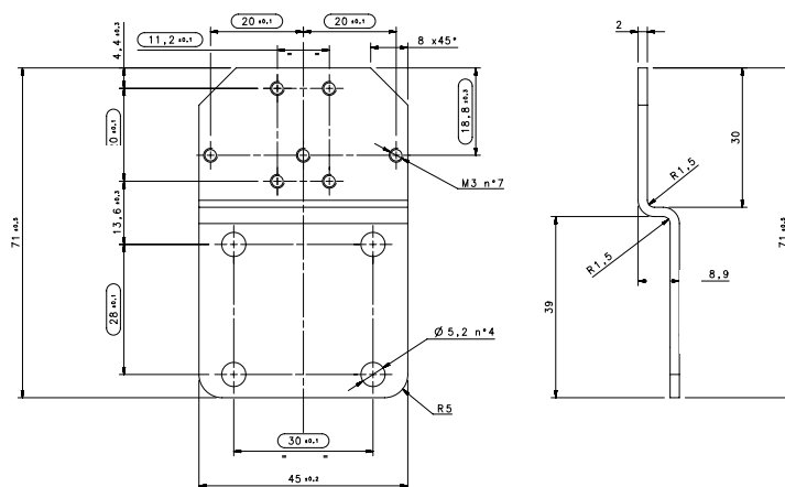
ST-S8-TL-LD46
