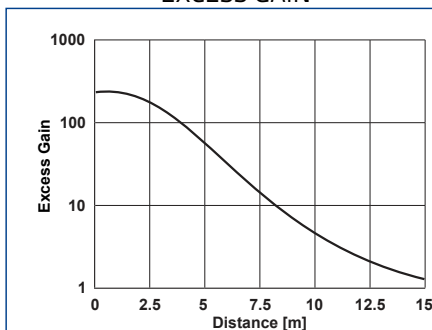
EXCESS GAIN
