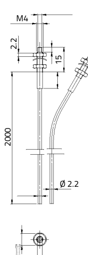
OF-43
