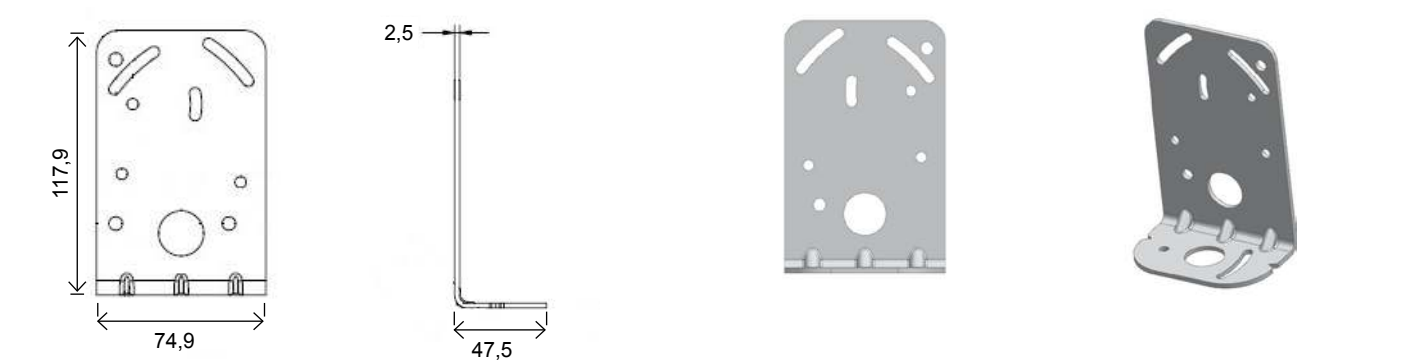
ST-S85-STD
