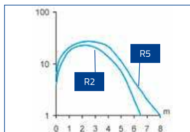
Excess gain
