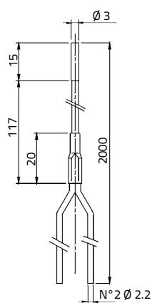
OF-38
