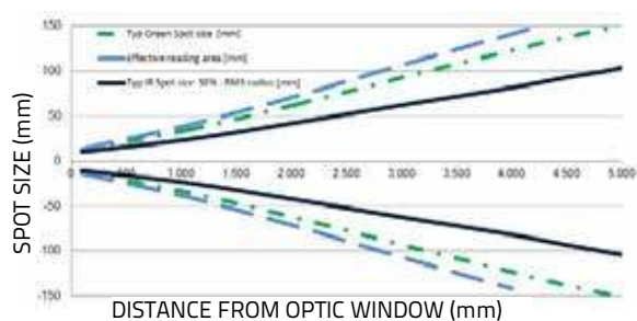
Typical spot size - squared section
