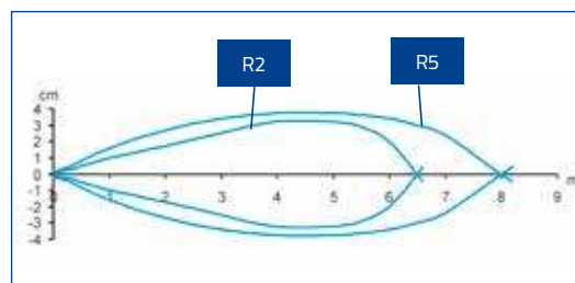
Detection area
