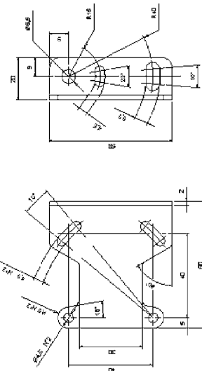
ST-504
