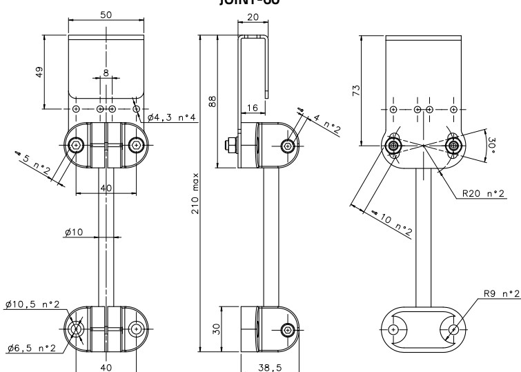
JOINT-60
