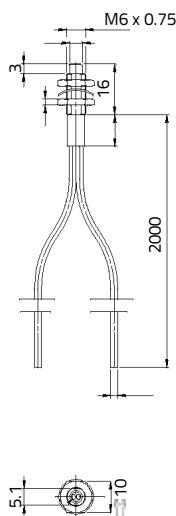
OF-42
