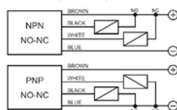
4 wires (NO+NC)
